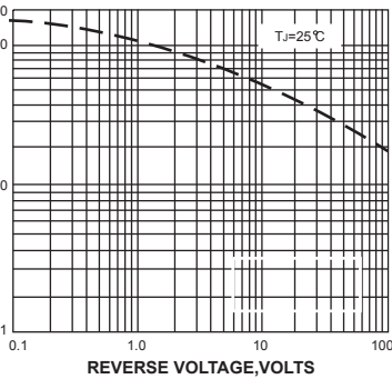
FIG. 5-TYPICAL JUNCTION CAPACITANCE
